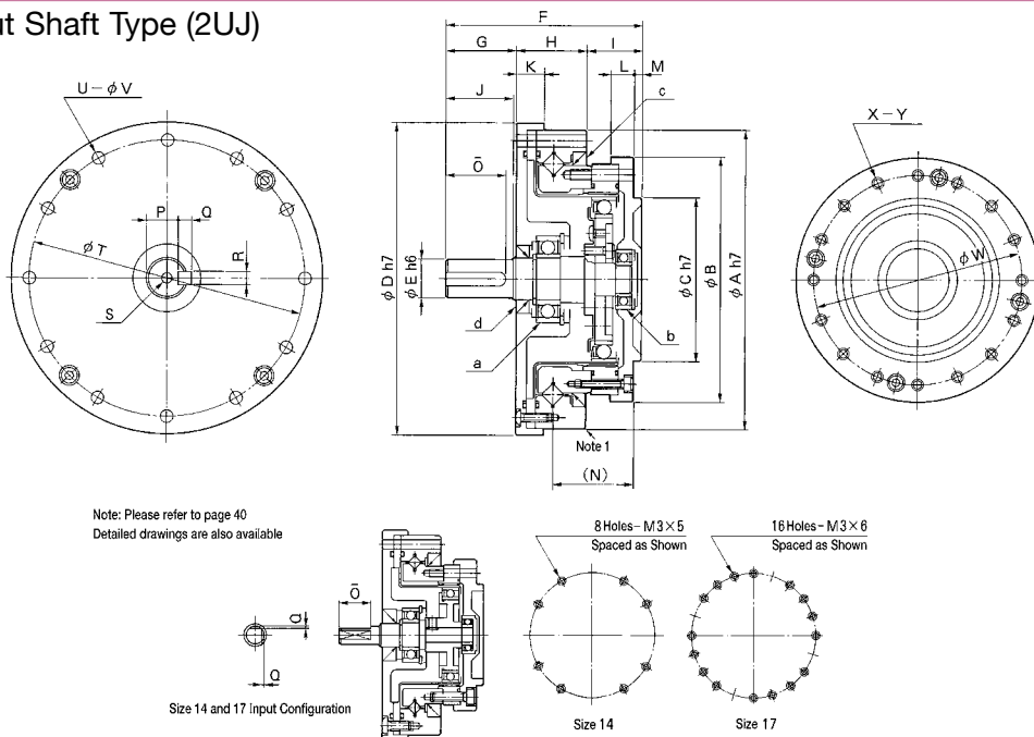
SHF SHG 2UJ Dimensions Table 24
