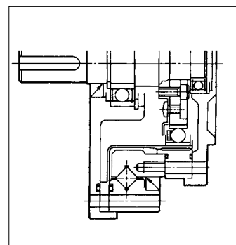
SIMPLE UNIT (2SH)
