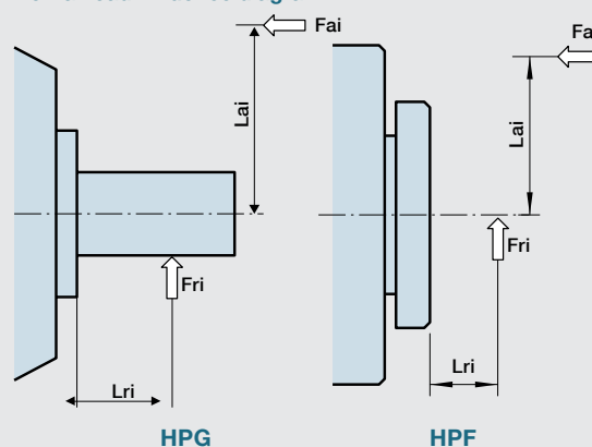
External load influence diagram
