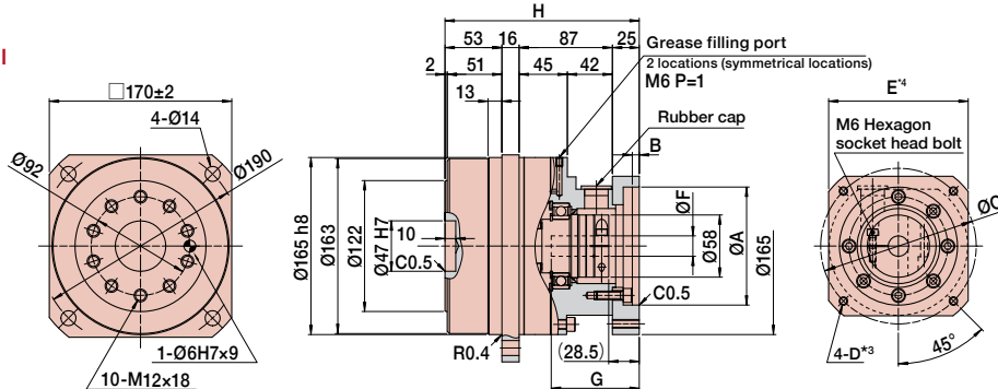
Flange Type II
