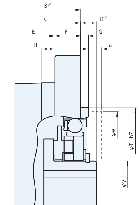
Detailed drawing for input side
