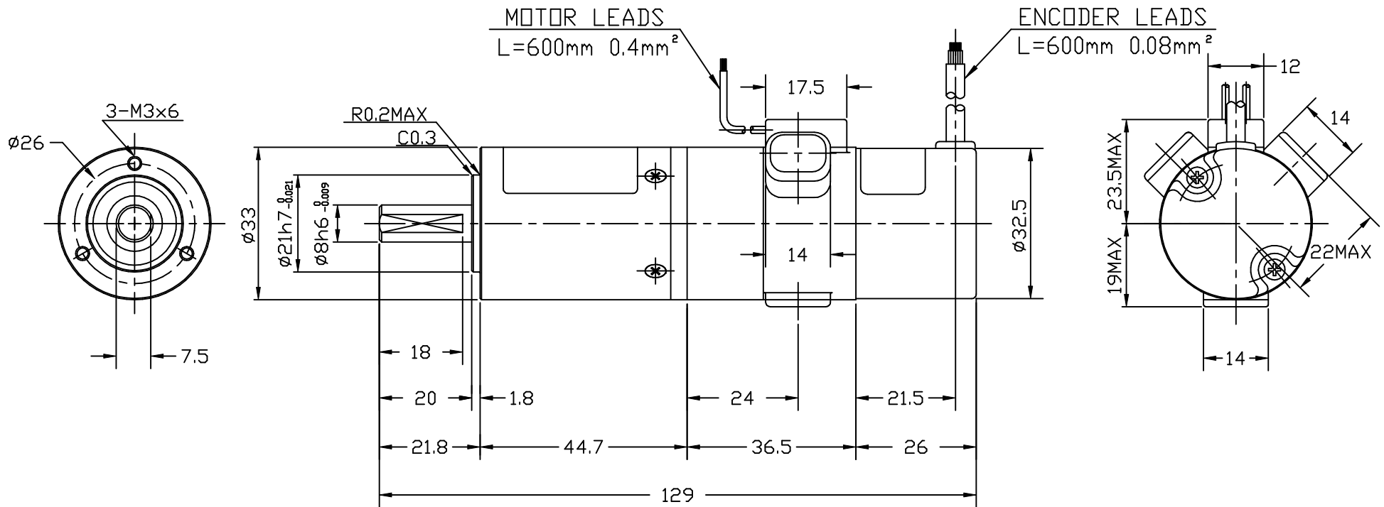
RH-8D-XX06-E100XX actuator with incremental encoder
